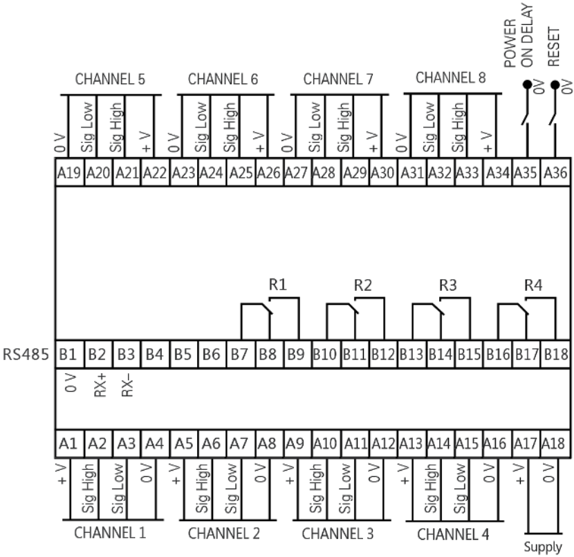
The output contacts are shown with the relays de-energised in the alarm condition
