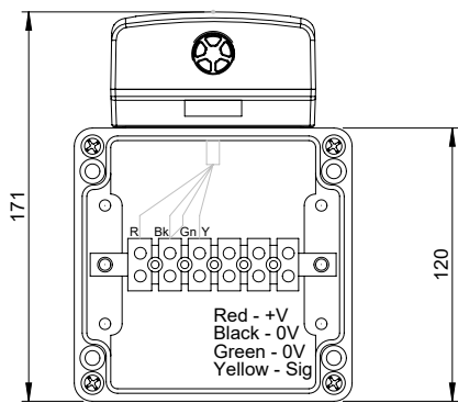
TX6831 with terminal box P5459.32
