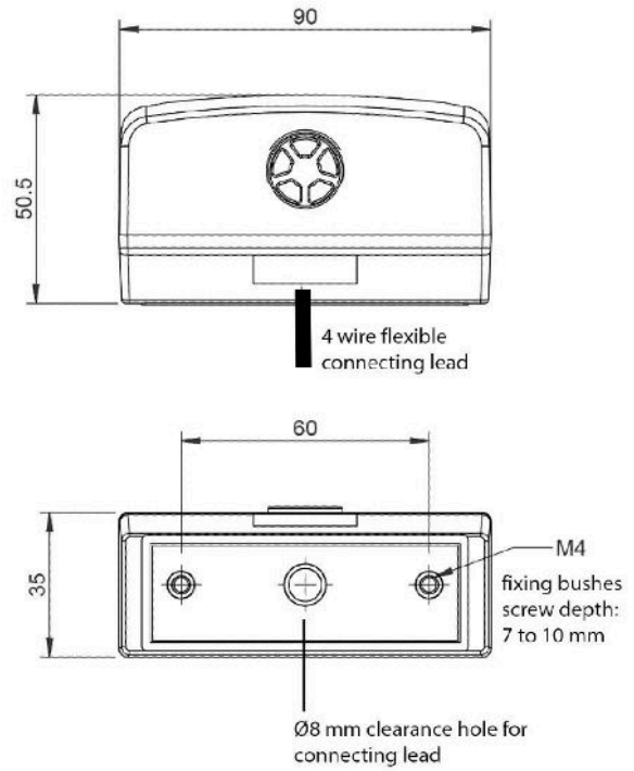
TX6831 with flexible lead for OEM applications
