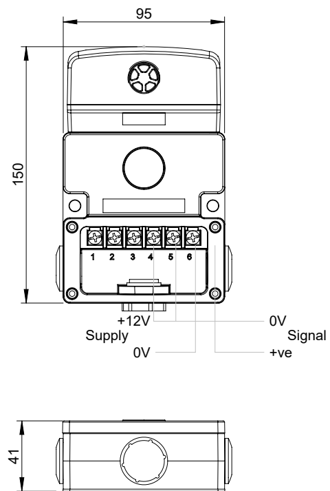
TX6831 with terminal box P5459.43
