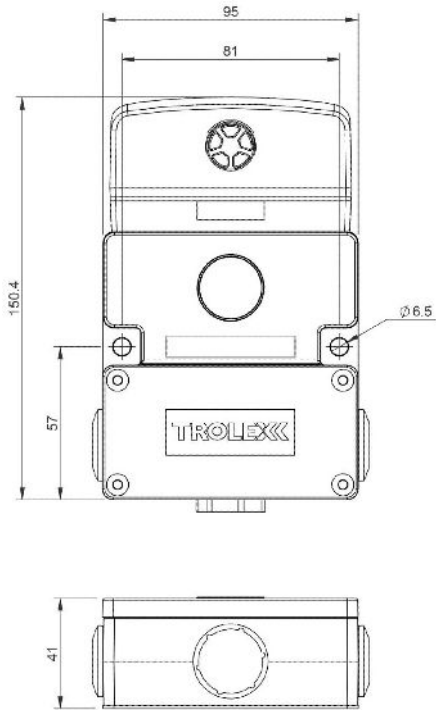
TX6831 with terminal box P5459.28
