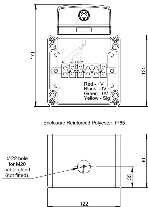
TX6831 with terminal box P5459.32
