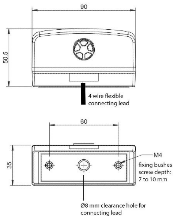
TX6831 with flexible lead for OEM applications
